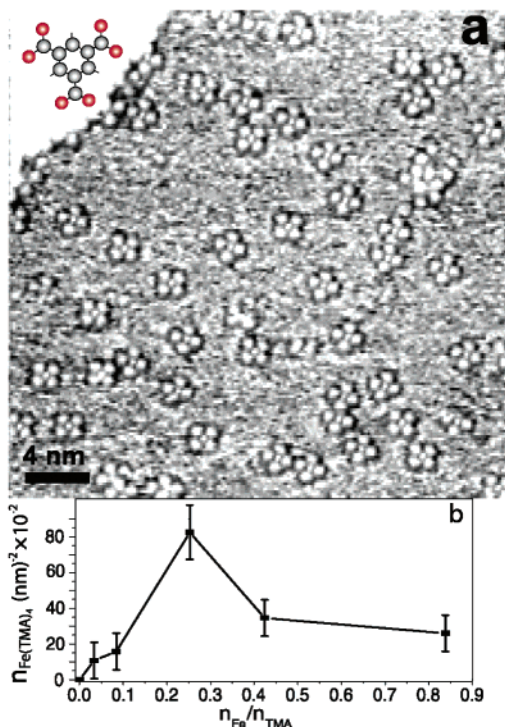
Figure 1. (a) Flower-shaped \text{Fe(TMA)}_4 complexes resolved by STM predominate on the Cu(100) surface following co-deposition of Fe and TMA in a 1:4 ratio at low coverages. The inset in the upper left shows a model of the TMA molecule (oxygen in red and carbon in gray; hydrogen omitted for clarity), which is imaged as an equilateral triangle in the STM image. (b) The evolution of the complex concentration as a function of the Fe–TMA concentration ratio (with the TMA coverage constant at 0.63 molecules per \text{nm}^2 ) has a marked peak at the ideal stoichiometry, where about 40% of the available reactants form \text{Fe(TMA)}_4 complexes.
